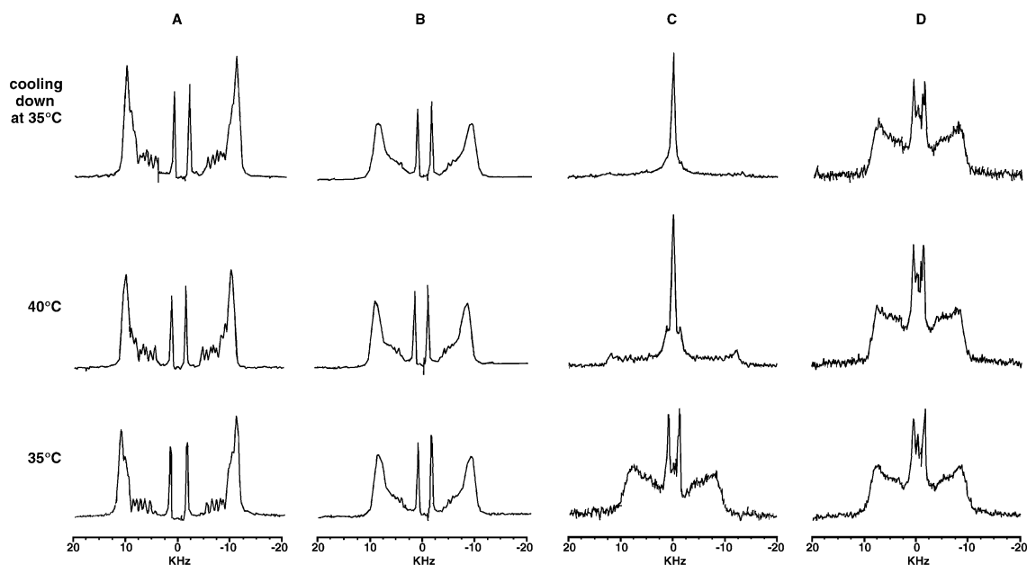
Fig. 7. ^2\text{H} NMR spectra of DMPC- \text{d}_{54} in DMPC/DHPC (3.5:1) bicelle solution at 35 and 40 °C and after cooling down at 35 °C. (A) Control bicelles; (B) Piracetam (200 mM) containing DMPC/DHPC bicelle solution; (C) Tyr-22–42 peptide containing bicelles (peptide/phospholipids 0.04); (D) Piracetam (200 mM) containing DMPC/DHPC bicelle solution submitted to the Tyr-22–42 peptide action (peptide/phospholipids 0.04).
